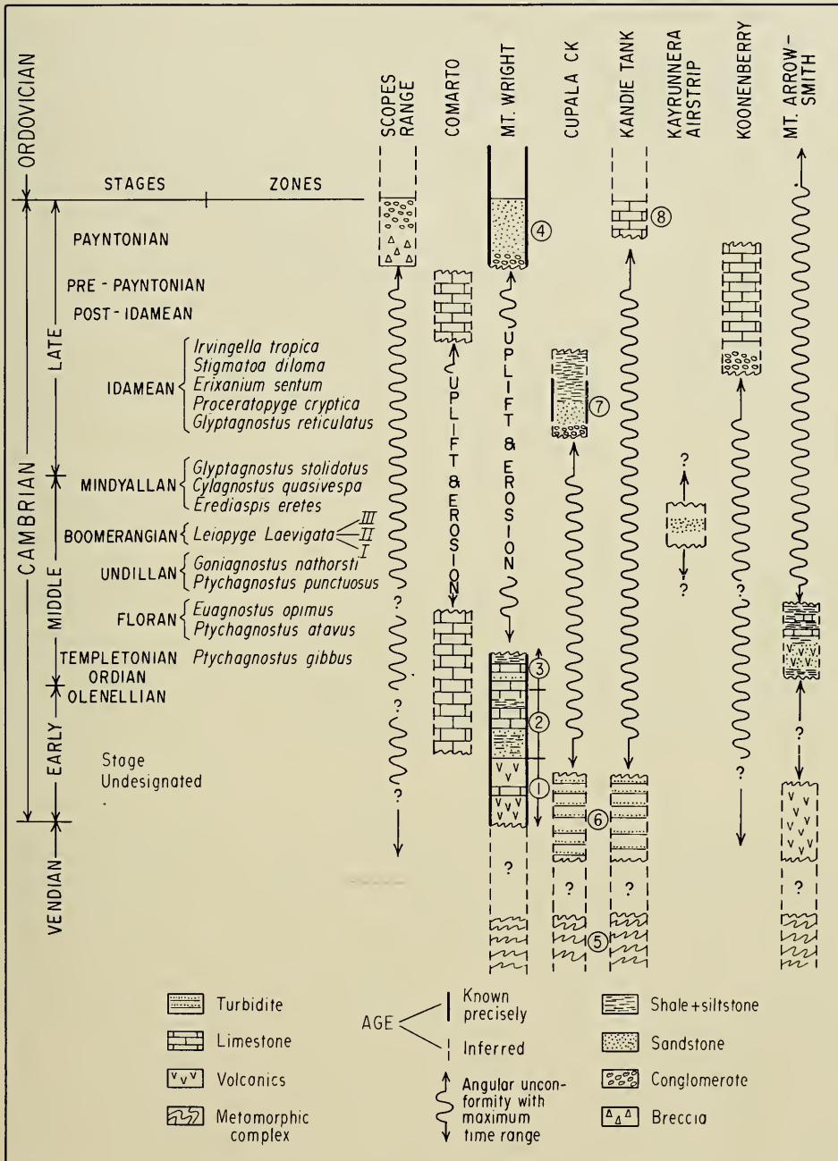
Fig. 9. Cambrian biostratigraphy of northwestern New South Wales, from Henderson (1976), Shergold (1971), and Öpik (1968). Age of Cambrian strata from Öpik (1968), Shergold (1971), Warris (1967), Wopfner (1966) and Jell (unpub. data). Circled numbers refer to the following formations. 1, Mount Wright Volcanics; 2, Cymbric Vale Formation; 3, Coonigan Formation; 4, Nootumbulla Sandstone; 5, Wonaminta Complex; 6, Copper Mine Range Beds; 7, Cupala Creek Formation; 8, Kandie Tank Limestone. Middle Cambrian is used in the sense of Öpik (1968), and Late Cambrian in the sense of Daily and Jago (1975).
